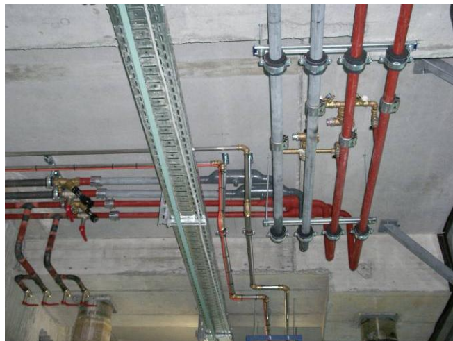
Supply lines beneath ceiling.
